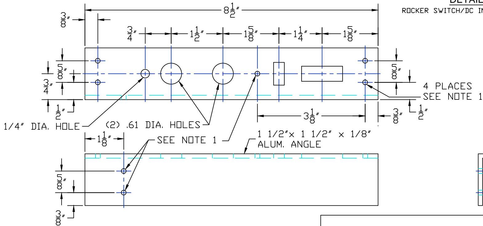
DETAIL-A
